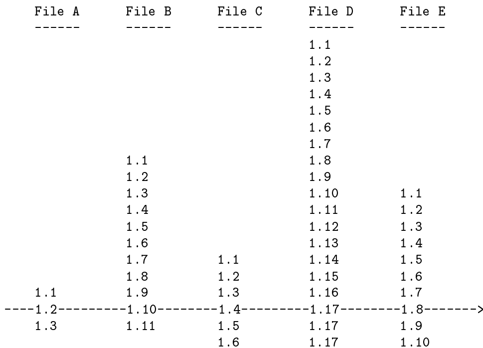
[Figure 2.2: The same tag as a "straight sight" through the revision history.]
