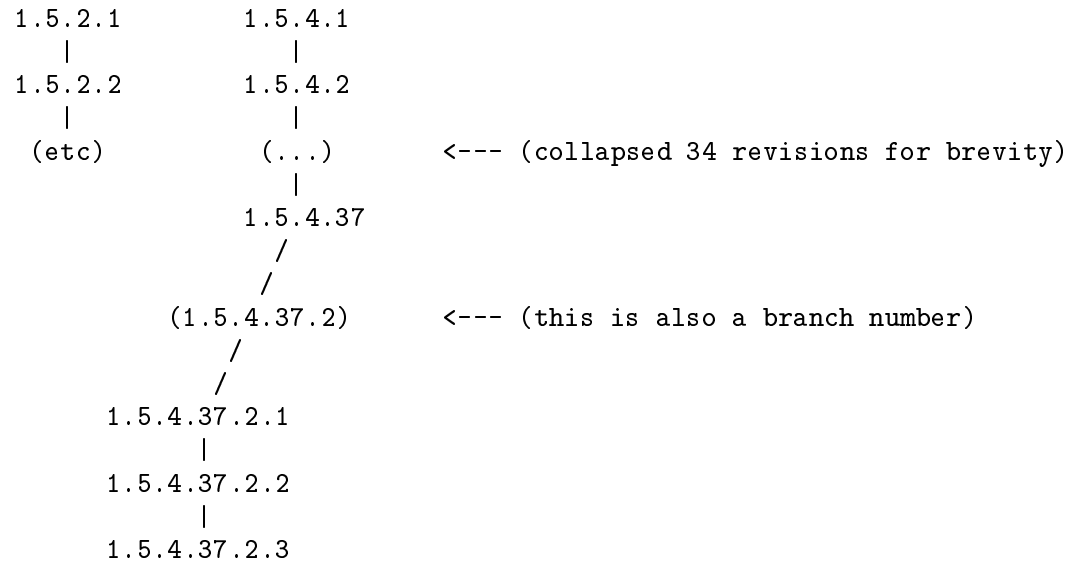
[Figure 2.4: An unusually high degree of branching. Time flows downward.]
